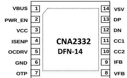
W-DFN3030-14
