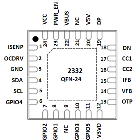
W-QFN4040-24
