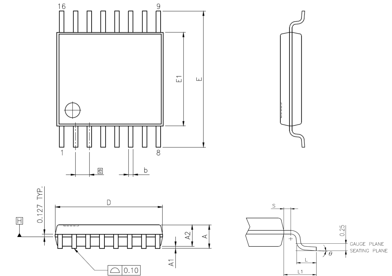
VARIATIONS (ALL DIMENSIONS SHOWN IN MM)
